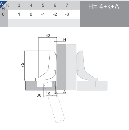
Damper *
