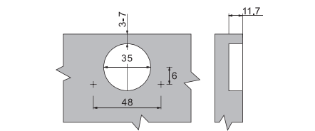
Screw mounting
