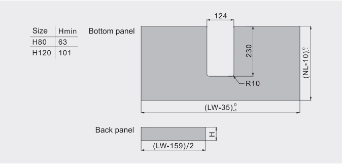
Magic box、 Regic box 16mm board cutting size
