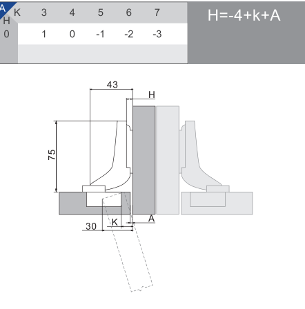
Bracket–Metal rebounder *
