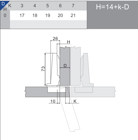
Screw mounting
