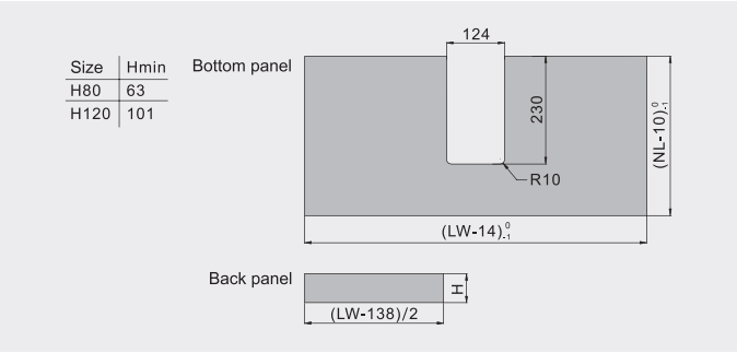
Cobox 16mm board cutting size
